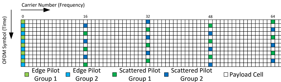
Figure L.11.23 MIMO pilot scheme MP16_2 for null pilot encoding.
