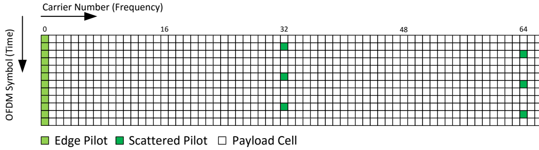
Figure E.1.16 Scattered pilot pattern SP32_4 (SISO, D_X = 32 , D_Y = 4 ).
