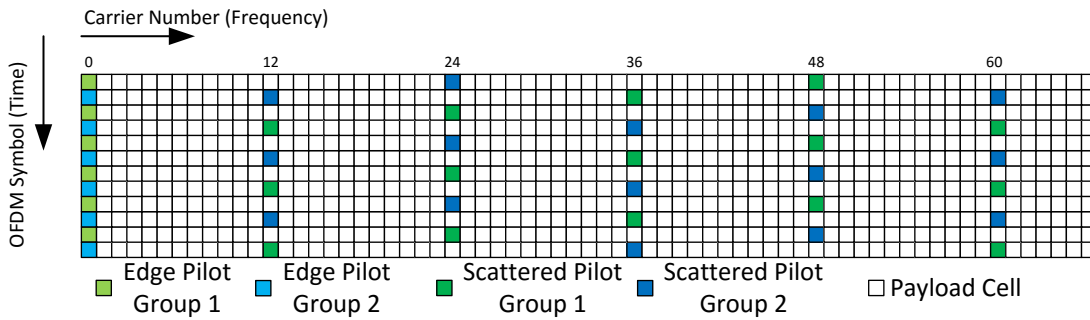
Figure L.11.21 MIMO pilot scheme MP12_2 for null pilot encoding.
