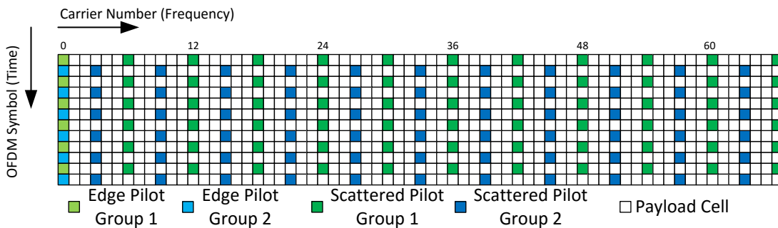
Figure L.11.1 MIMO pilot scheme MP3_2 for Walsh-Hadamard pilot encoding.
